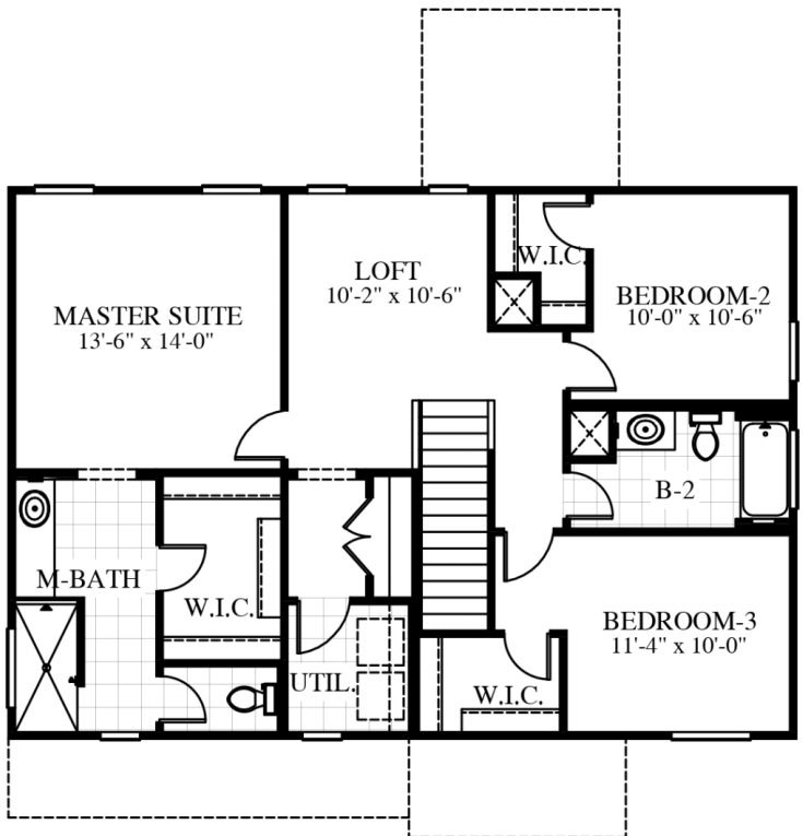
SECOND FLOOR
