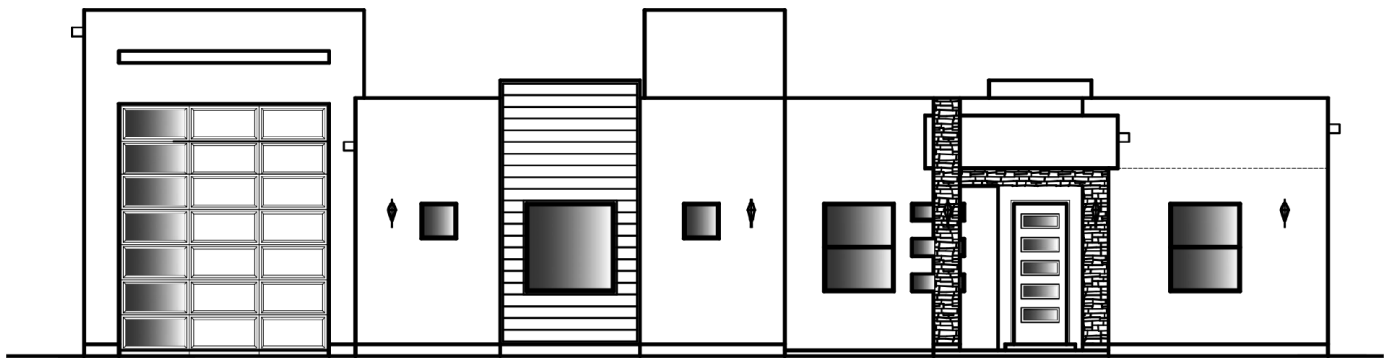
DESERT MODERN ELEVATION Elevation shown with optional RV Garage
