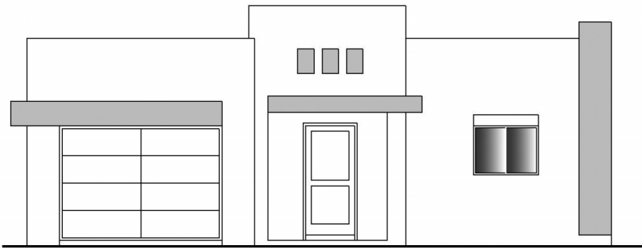
ELEVATION C
