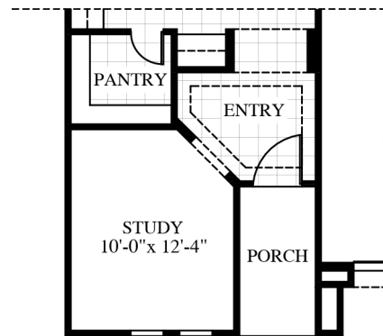
FLOORPLAN ELEVATION C
