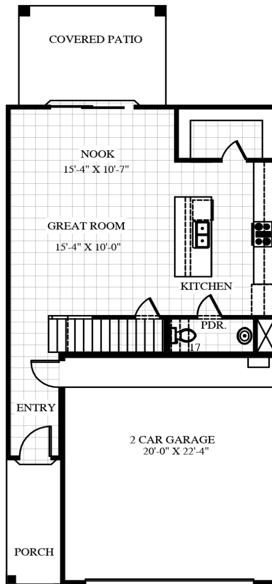
FIRST FLOOR
